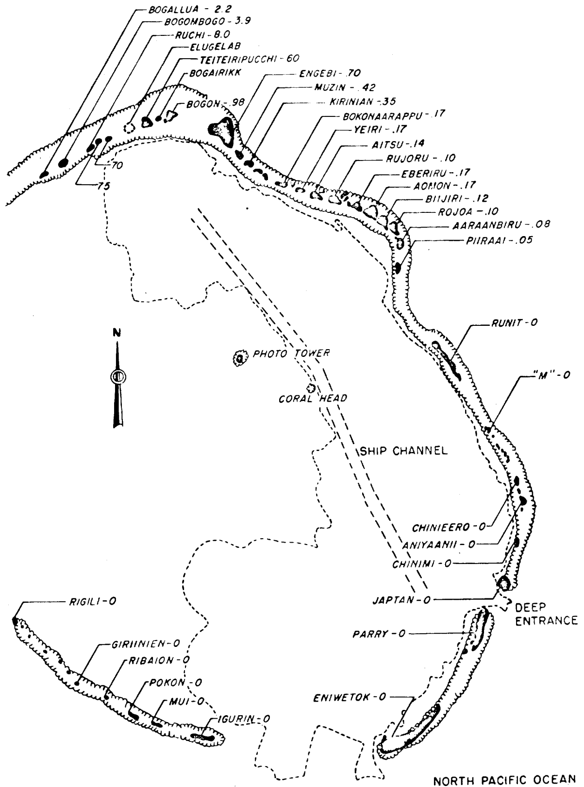
Fig. 4.13 NECTAR radiation intensities in roentgens per hour extrapolated to H + 4 hr. Location, Elugelab crater (barge). Yield, 1.7 Mt. Time fired, 14/0620M May 1954.
